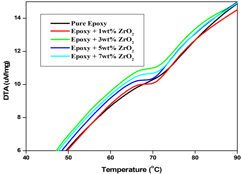
FIG. 5. DTA curve of pure and ZrO 2 added nanocomposites.
