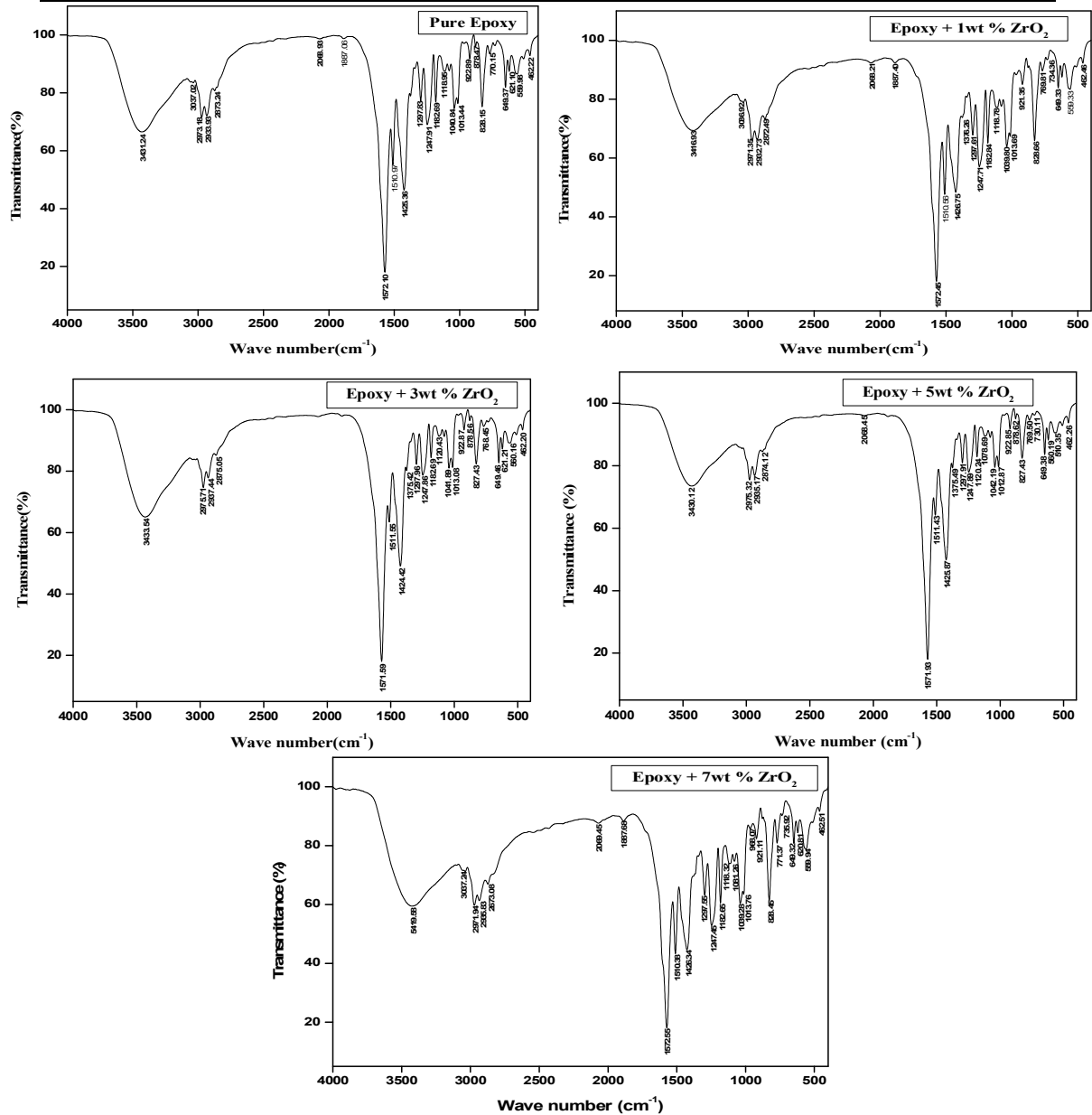
FIG. 3. FTIR spectra of pure epoxy and ZrO 2 -epoxy nanocomposites.
