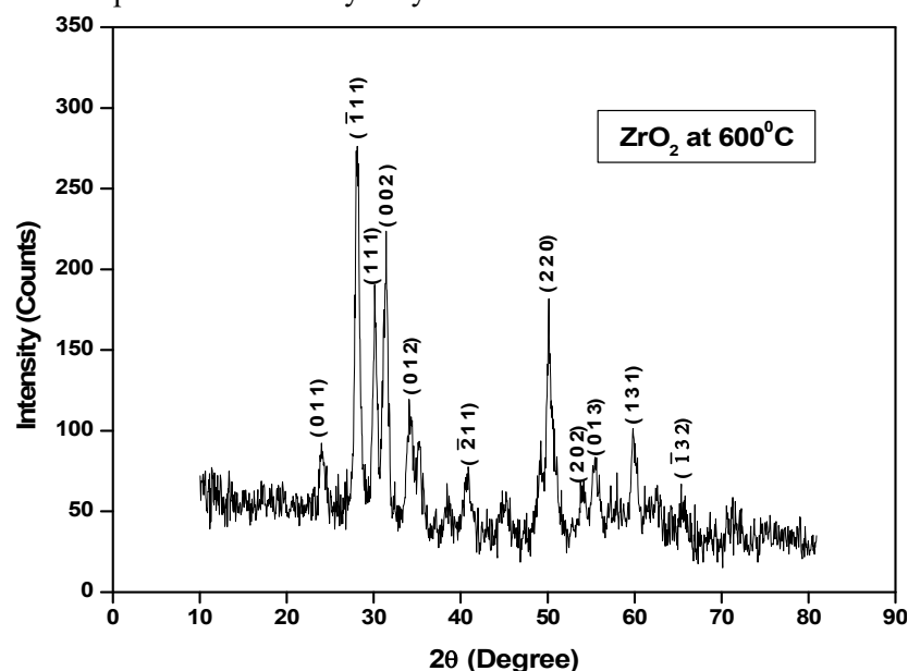
FIG. 2. XRD pattern of \text{ZrO}_2 nanoparticle.
